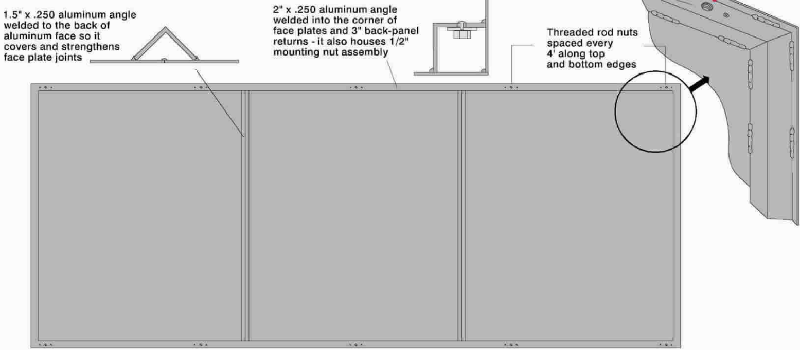
Back structural and mounting hardware details
