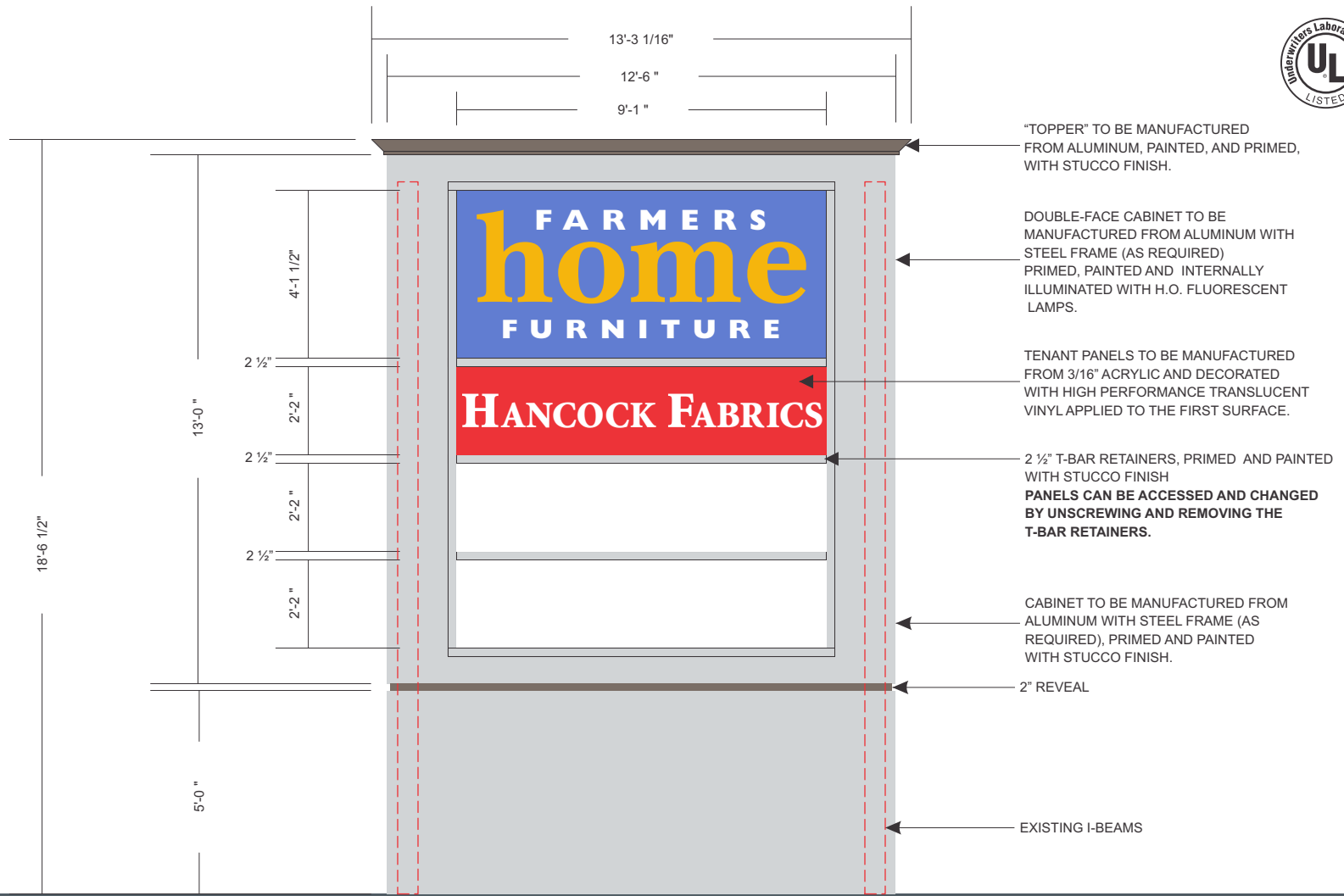
1 A MONUMENT SIGN - FRONT SCALE: 1/4" = 1'-0"
