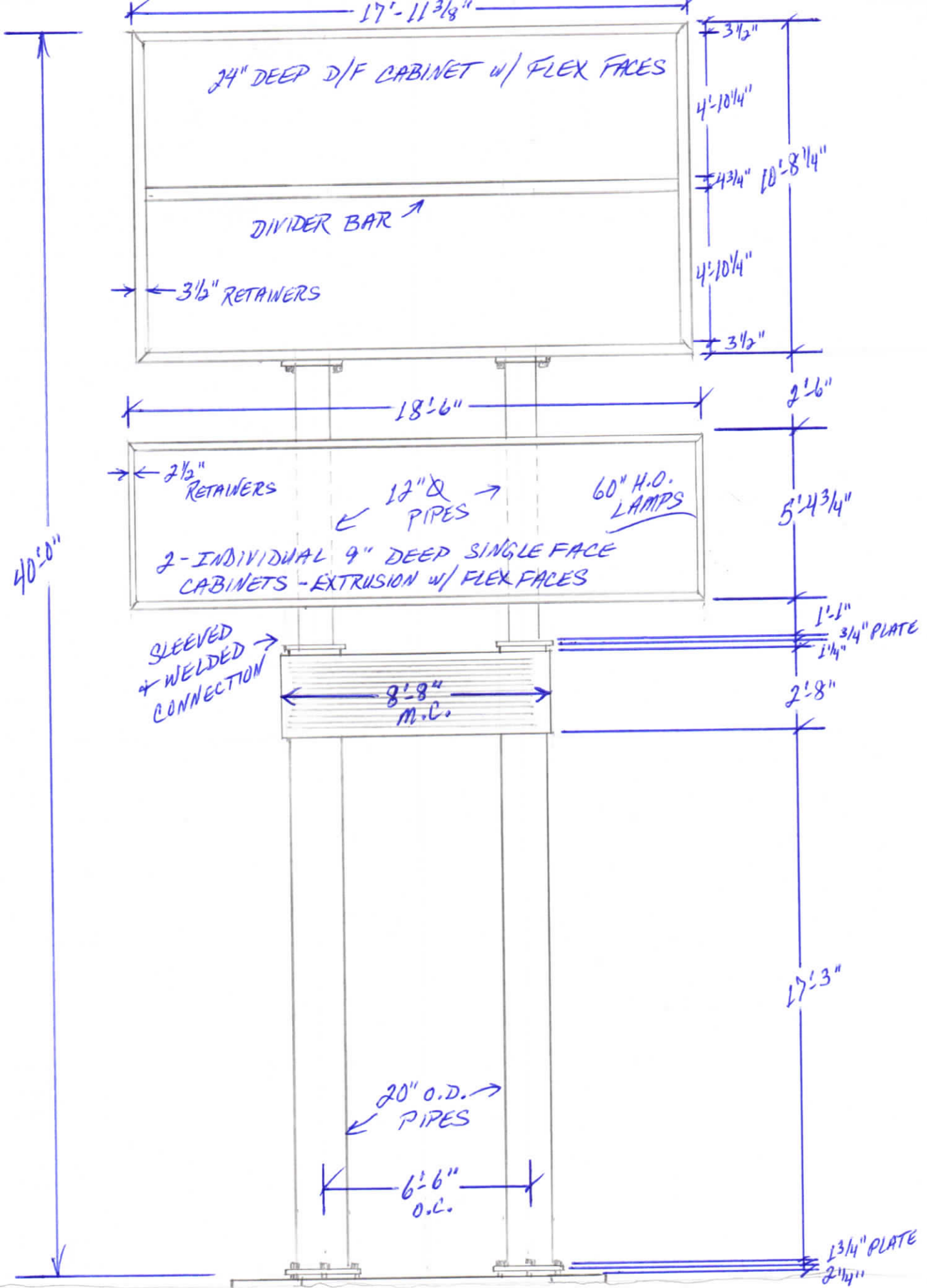
1 3/4" x 28" x 28" BASE PLATES w/ 6-1" DIA. ANCHOR BOLTS 12" O.C.
